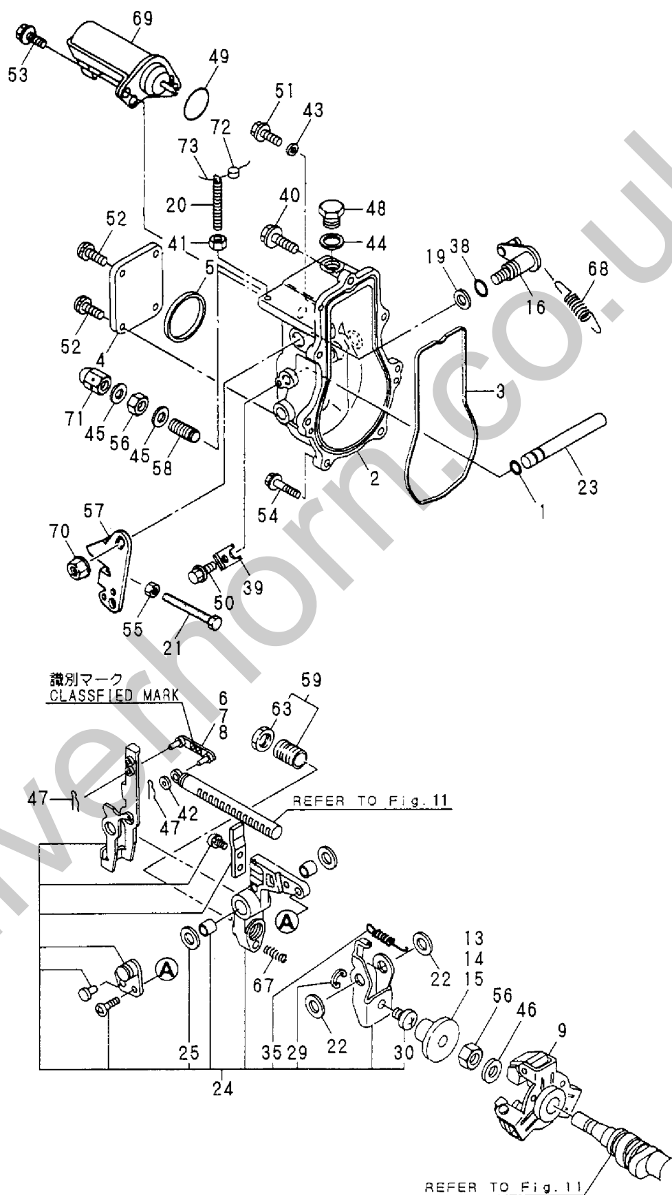
Fig. 12 ガバナ GOVERNOR
